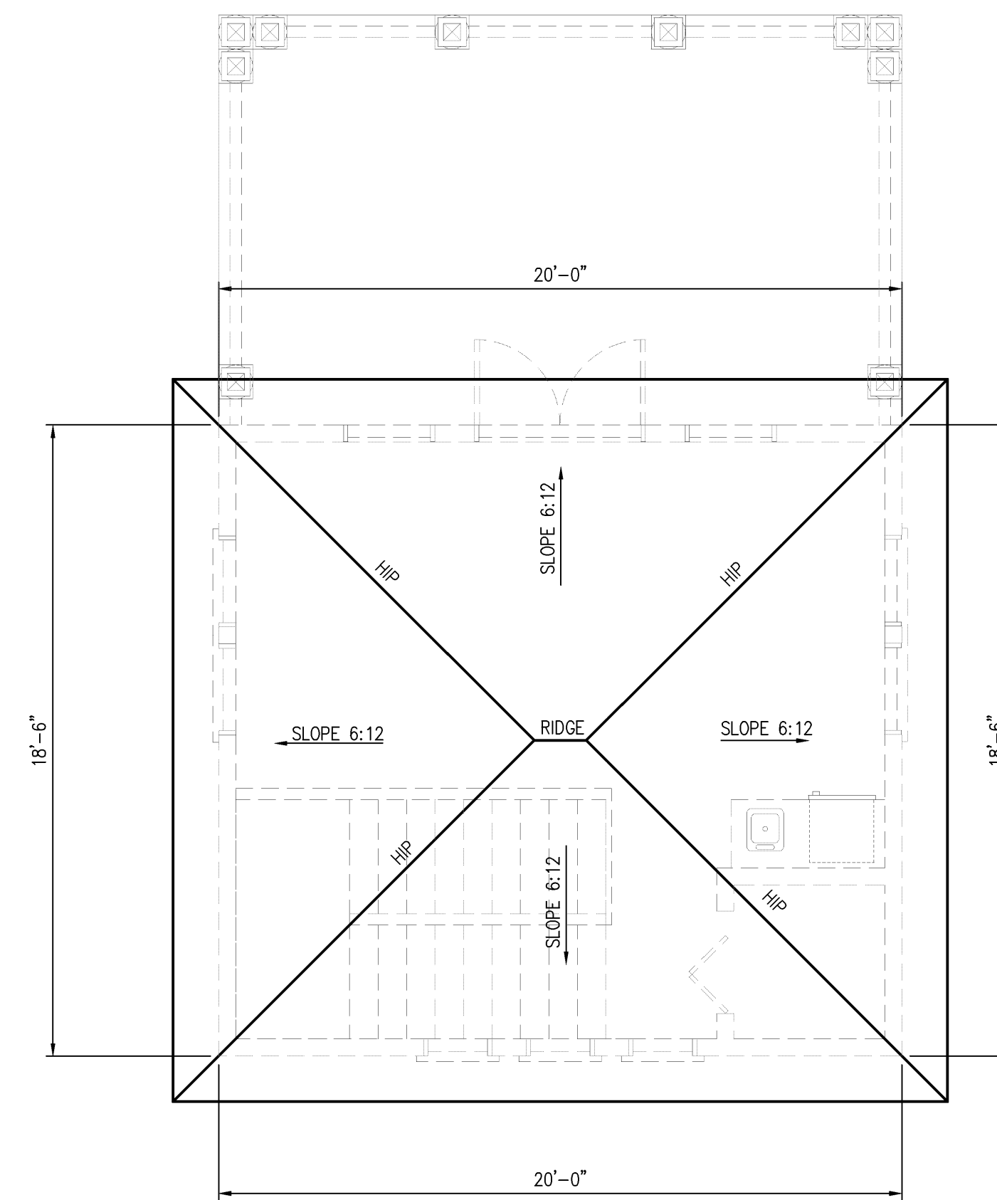
FOURTH FLOOR ROOF PLAN
